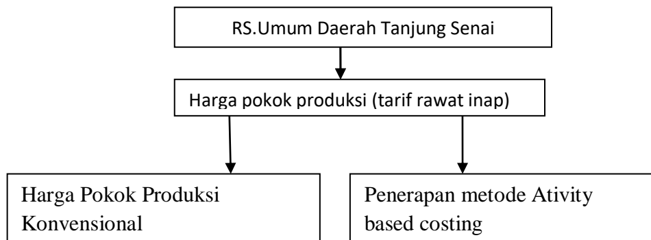
Gambar I.1 Paradigma Penelitian
