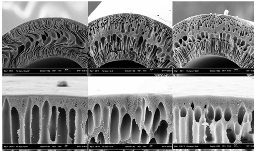
Fig. 4. Cross section and outer surface FESEM images of the modified
