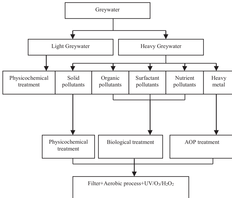
Fig. 1. The greywater technology treatment for aquaculture safety.
