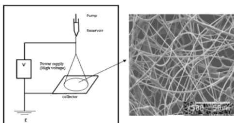
Figure 1 Electrospinning principle and resulting of nanofiber mat (SEM picture)
