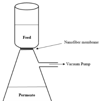
Figure 2 Illustration of nanofibre membrane filtration set up for stand-alone
