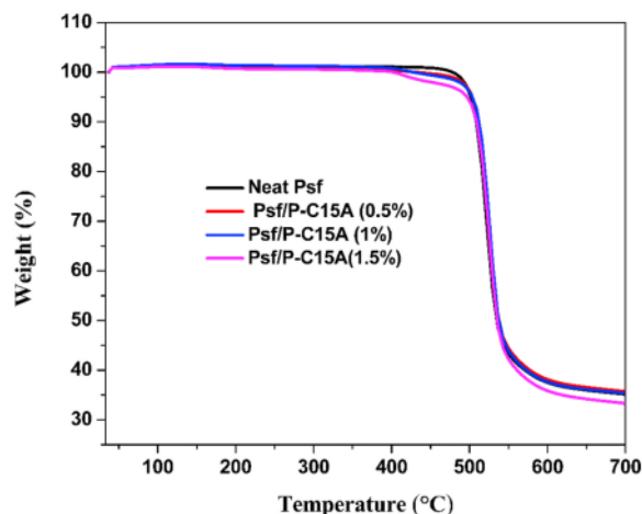
Fig. 8. TGA analysis of neat and PSf/P-C15A MMMs.
