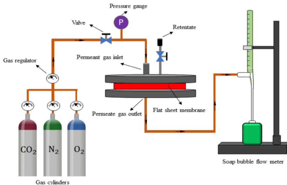
Fig. 3. Gas permeation testing setup.
