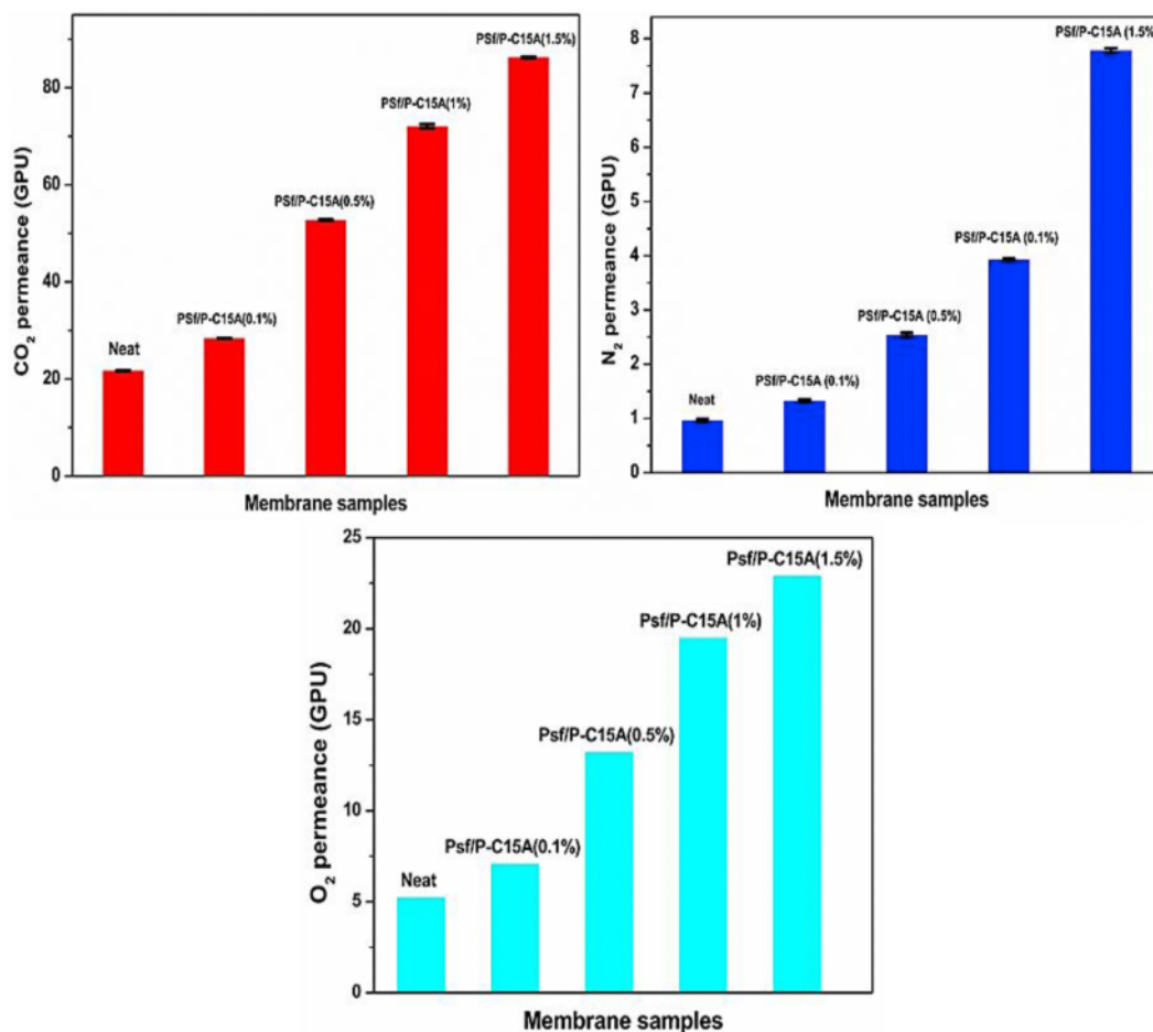
Fig. 10. Permeance of neat and PSf/P-C15A MMMs.
