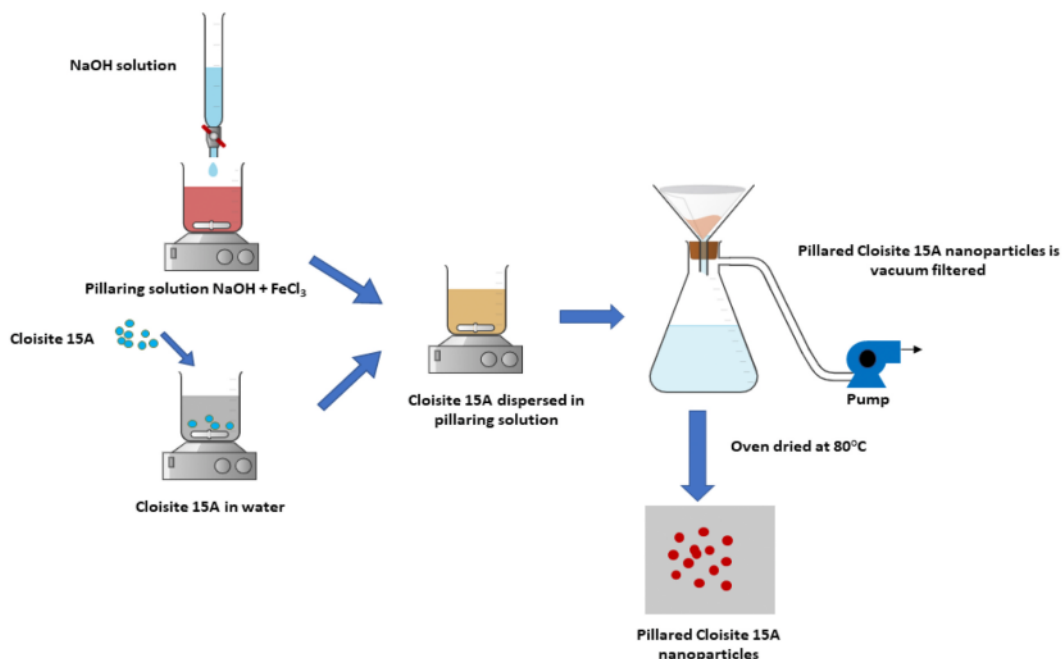
Fig. 1. Schematic representation of pillared cloisite 15A synthesis.
