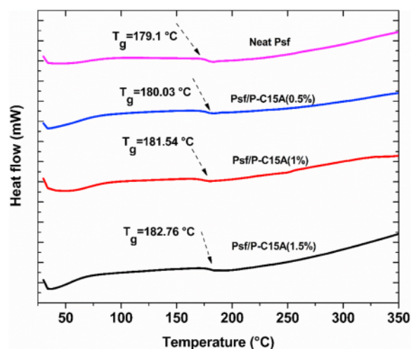
Fig. 9. DSC thermographs of neat and PSf/P-C15A MMMs.
