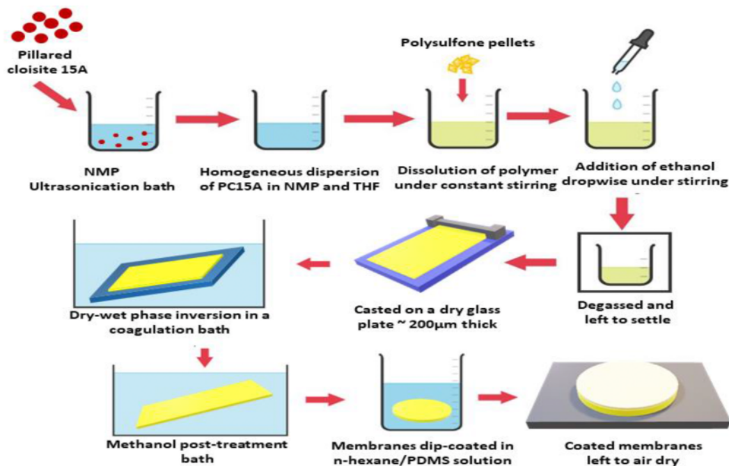
Fig. 2. Schematic representation of membrane casting procedure.
