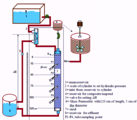
Fig 1. Packed Column Remediation
