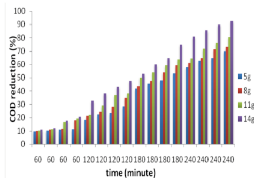
Fig.3. Effect of concentration of composite and contact time on COD reduction
