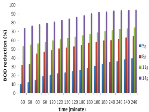
Fig.2. Effect of concentration of composite and contact time on BOD 5 reduction
