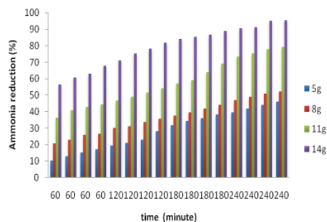
Fig.4. Effect of concentration of composite and contact time on ammonia reduction
