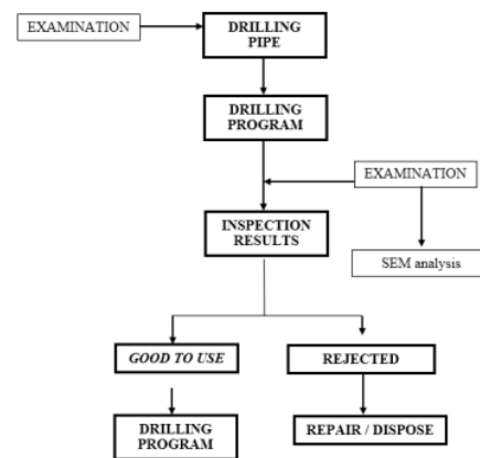
Figure 1. Research Flowchart
