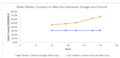
Figure 1 : Ratio Water Content in Wet Gas between Design and Actual
