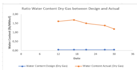
Figure 2 : Ratio Water Content in Dry Gas between Design and Actual
