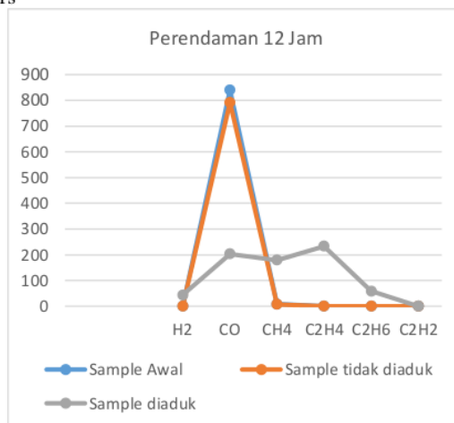
Figure 2. Graph of gas absorption after soaking for 12 hours.
