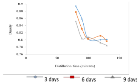
Fig.10: Fermentation time vs density of 12 gram yeast weight Graph
